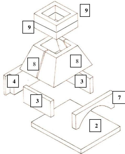
Figure 2. Vecchio™ Pizza Oven Components
