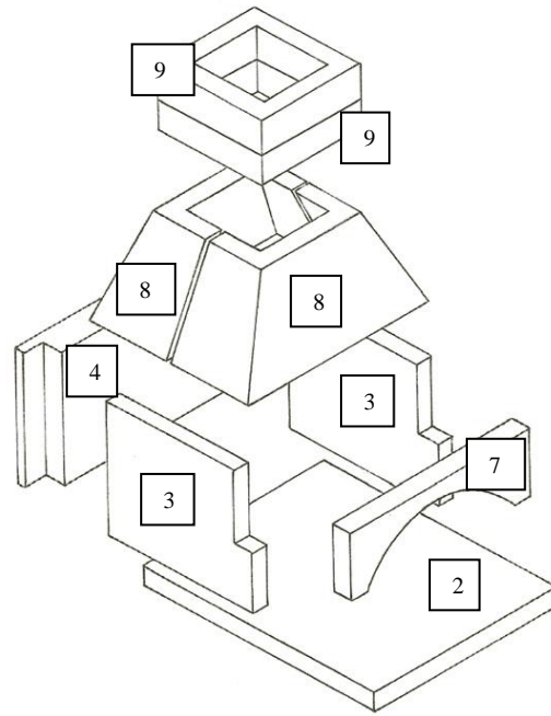
Figure 5. Oven Components
