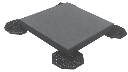
18x18 Heritage Slab with 7X Stackable Pedestal
